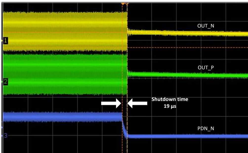
Figure 16: Shutdown timing (19 µs from de-asserting PDN_N to zero output)
