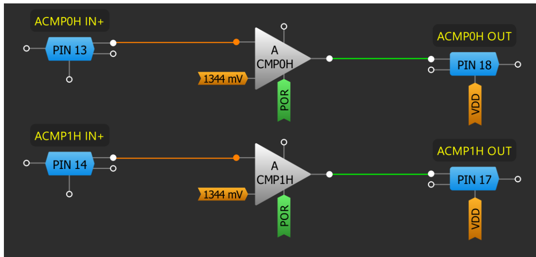
Figure 5: Testing Design
