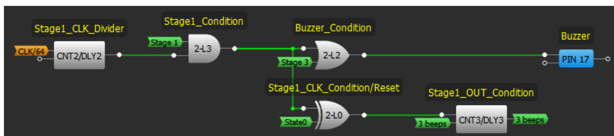
Figure 2. Stage 1 Section
