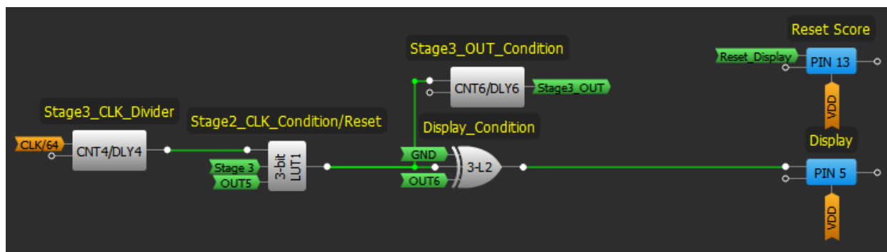
Figure 5. Stage 3 Section
