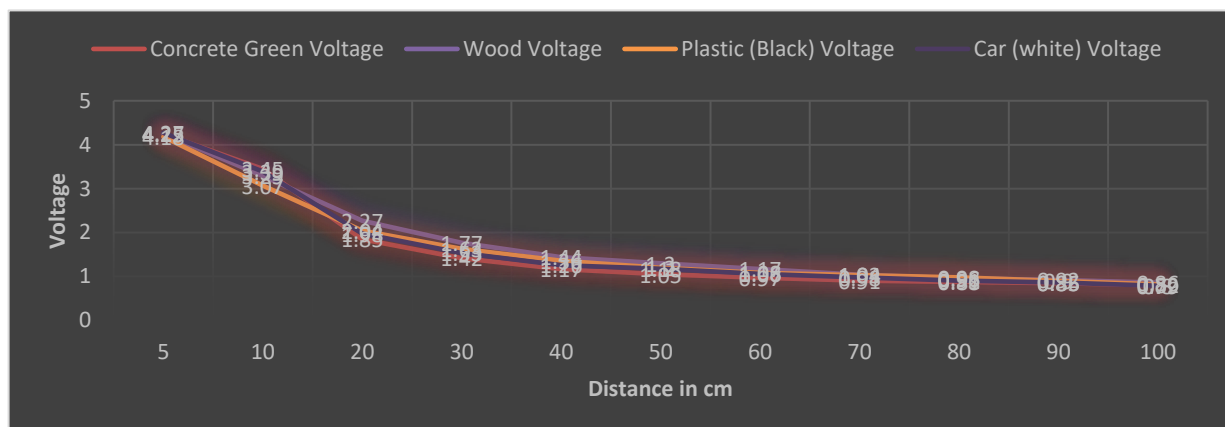
Figure 3. GP2Y0A60SZLF Voltage/Distance Curve
