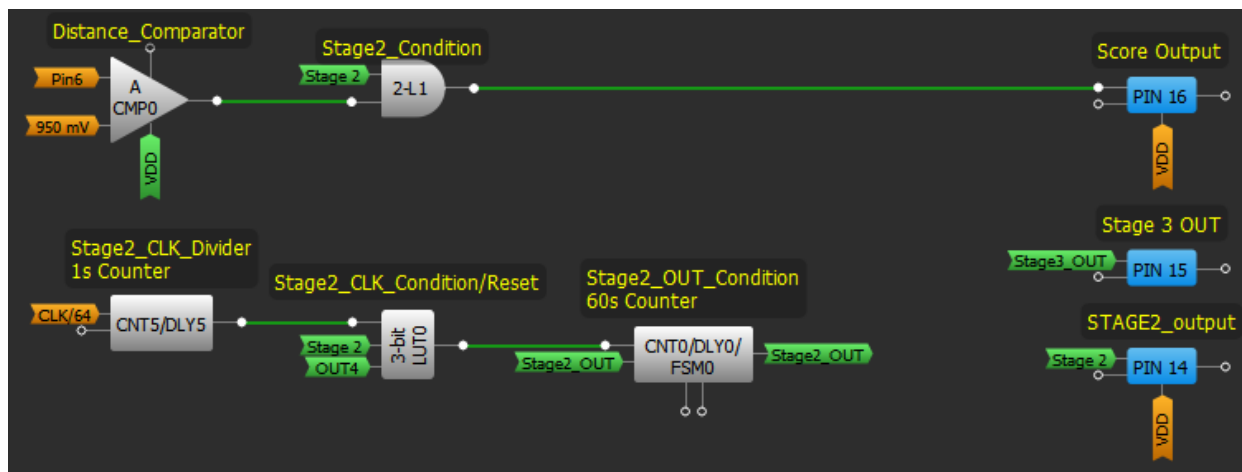
Figure 4. Stage 2 Section
