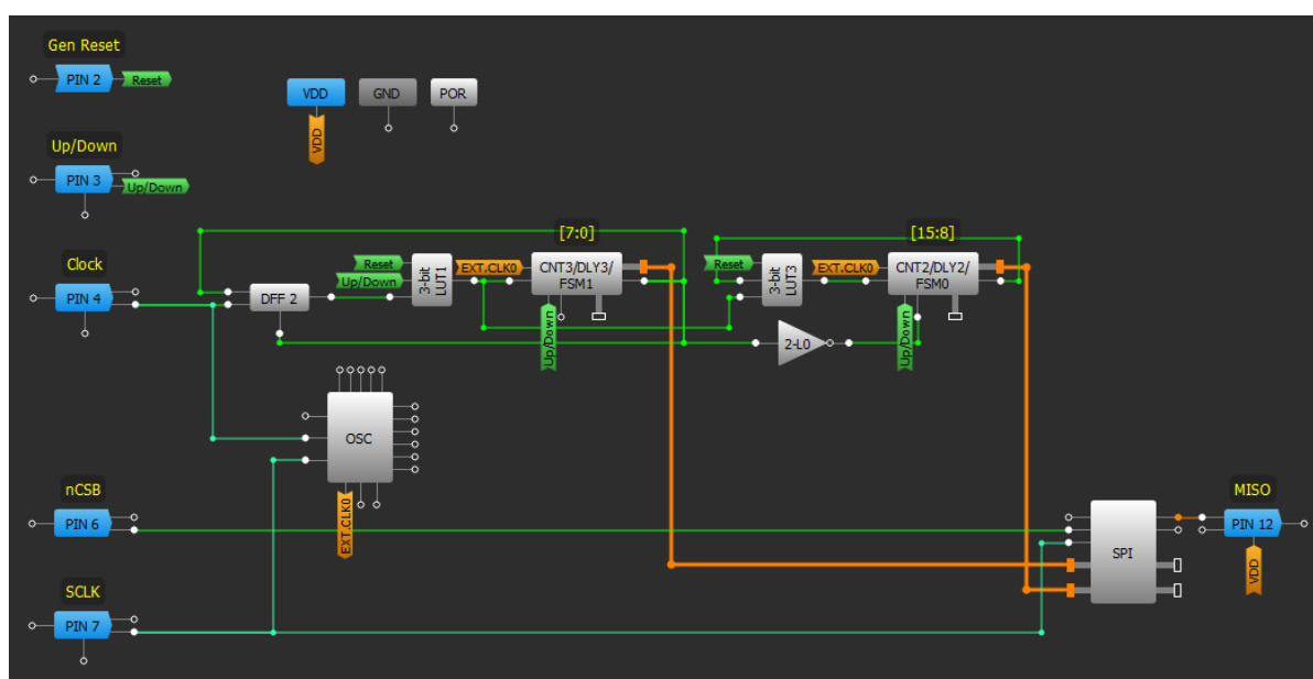
Figure 1: "16-bit FSM with SPI Output"
