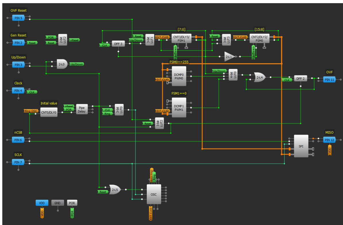
Figure 3: "16-bit FSM with SPI Output, OVF and Initial Value's Setting Functions"
