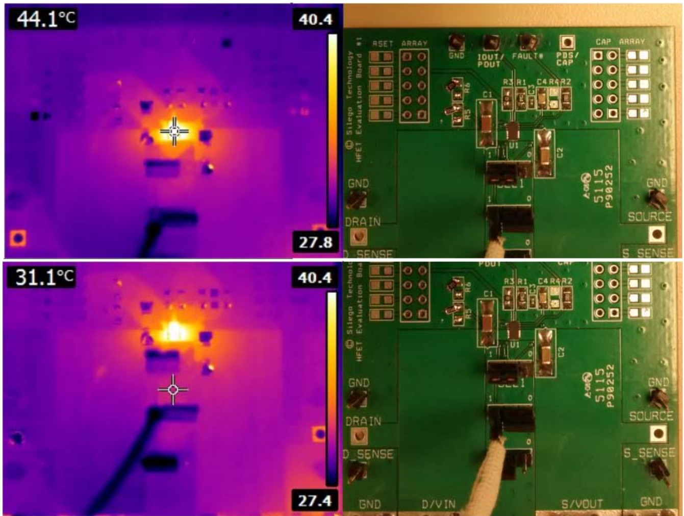
Figure 4. Thermal distribution for V_{IN} = 20\text{ V} , I_{DS} = 4.5\text{ A} after 2 min power up
