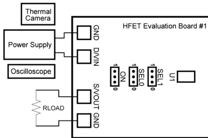
Figure 3. SLG59H1007V Evaluation Board Connection Circuit
