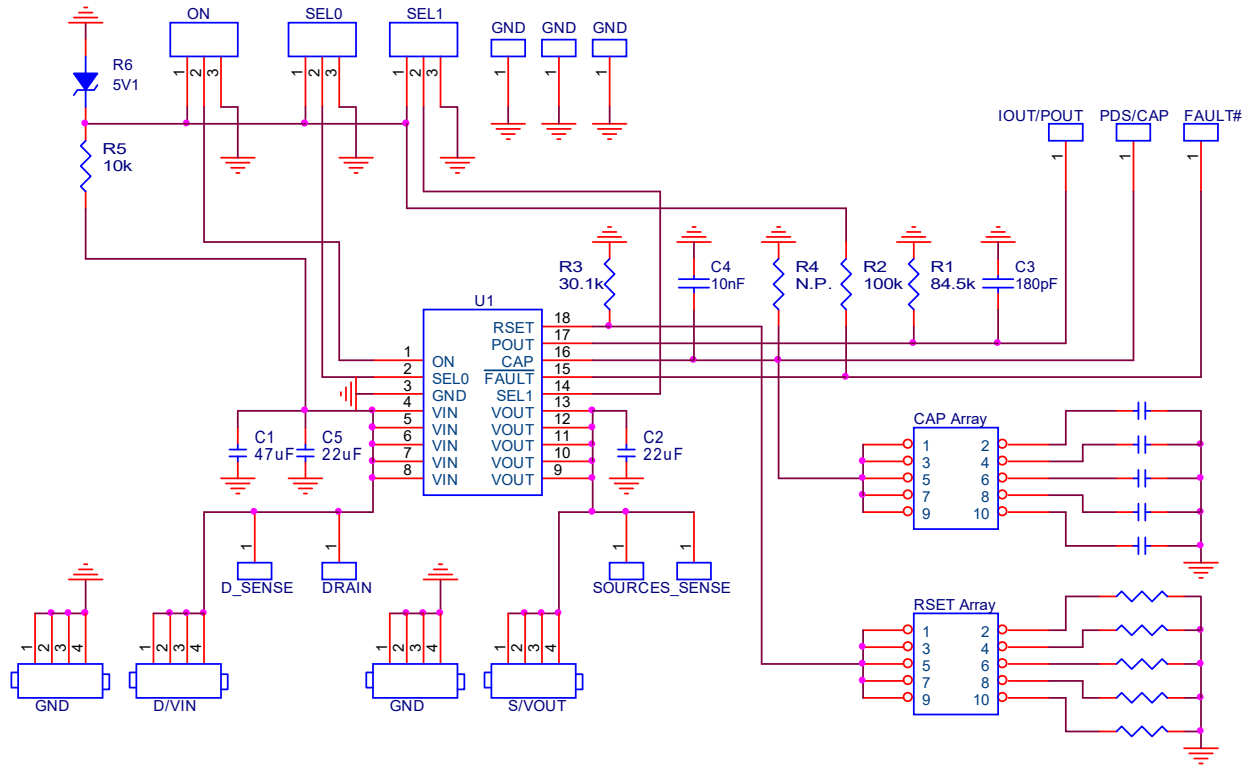
Figure 2. SLG59H1007V Evaluation Board Connection Circuit
