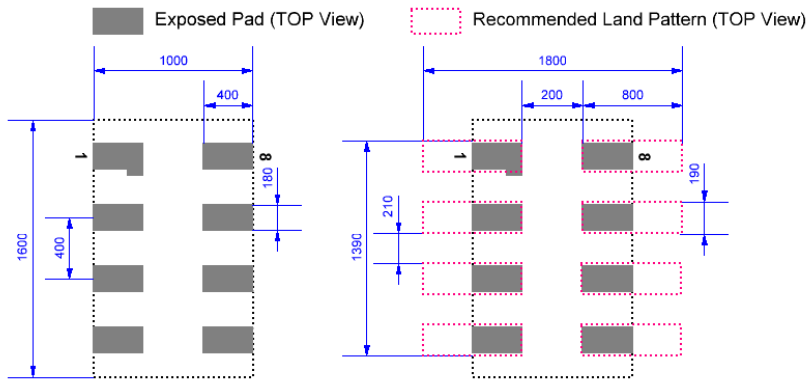
Figure 2. SLG59M1640V Package Dimensions and Recommended Land Pattern
