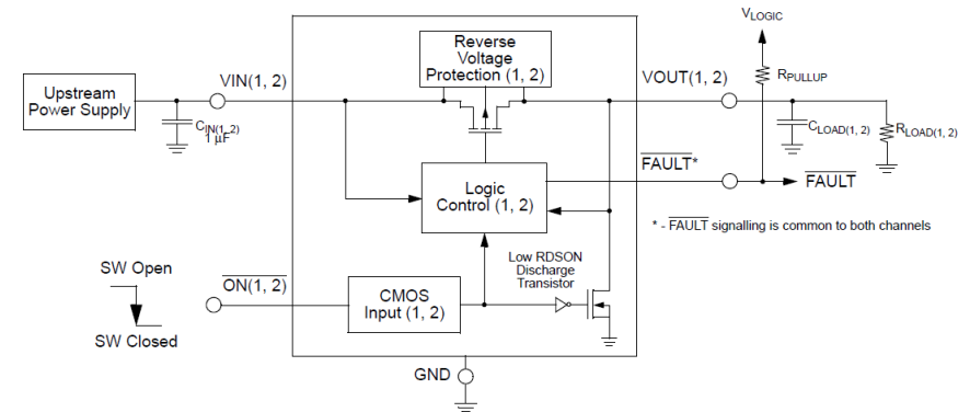
Figure 1: SLG59M1640V Block Diagram
