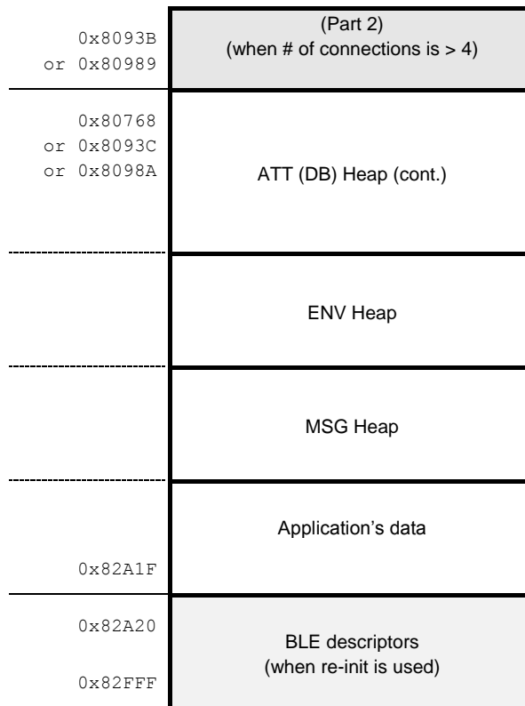
Figure 19: Extended Sleep layout in 0x80000 to 0x82FFF
