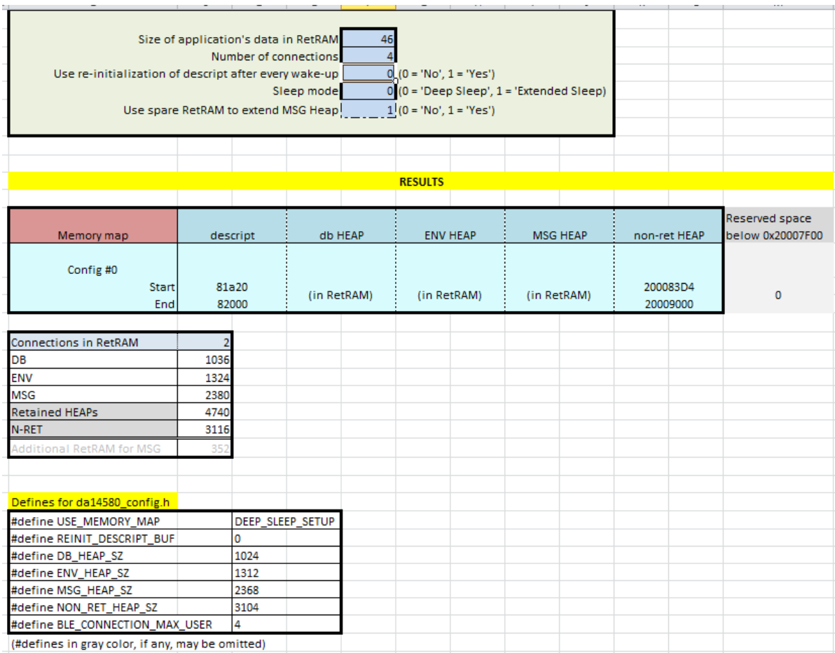
Figure 10: Master with 4 connections without re-initialization of descriptors
