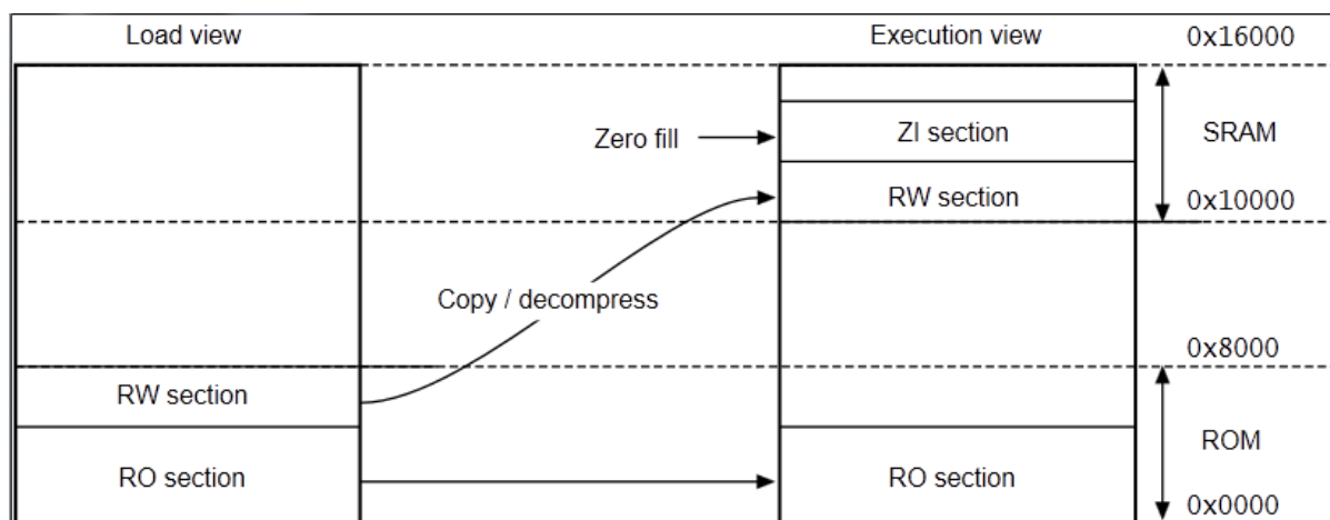
Figure 3: Load and Execution Regions 3
