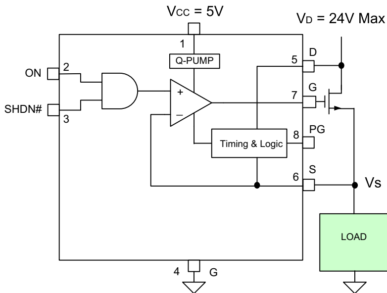
SLG5NT021 For N-MOSFETS with V_{GS} < 20V
